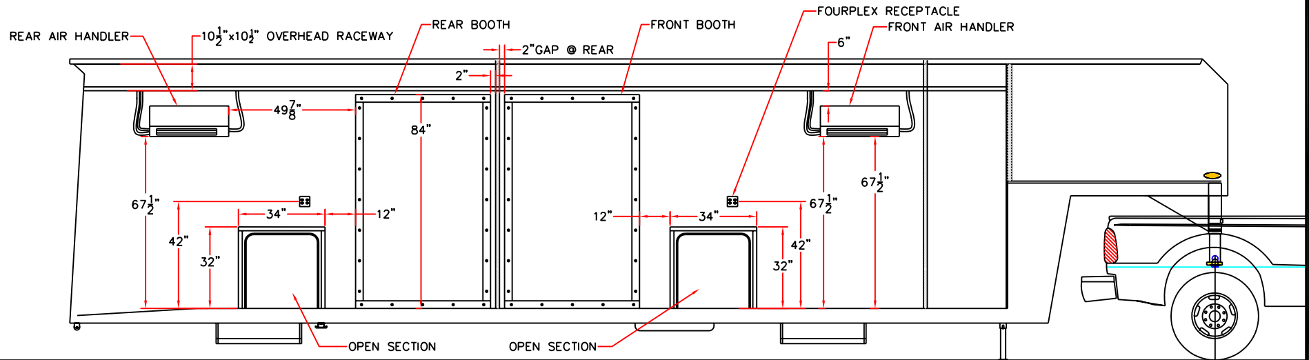
INTERIOR VIEW OF DESK PLACEMENT AGAINST THE DRIVER'S SIDEWALL
